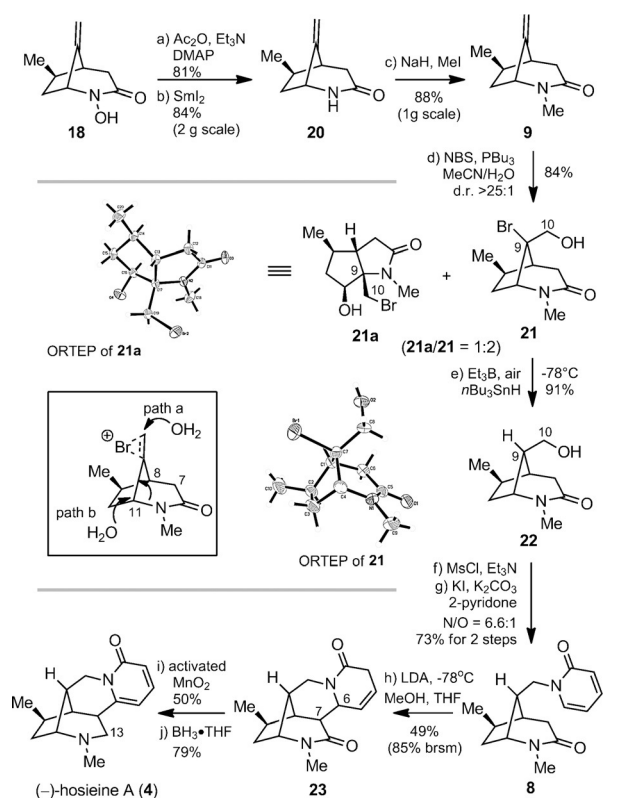
Scheme 4. Complete synthesis of (–)-hosieine A ( 4 ). a) \text{Ac}_2\text{O} (1.2 equiv), \text{Et}_3\text{N} (1.3 equiv), DMAP (cat.), RT, 45 min, 81%. b) \text{SmI}_2 (2.4 equiv), THF, RT, 20 min, 84%. c) \text{NaH} (1.2 equiv), \text{MeI} (1.5 equiv), THF/DMF (2:1), RT, 1 h, 88%. d) \text{NBS} (1.5 equiv), \text{PBu}_3 (0.4 equiv), \text{MeCN}/\text{H}_2\text{O} (5:3), 0^\circ\text{C} , 84% ( 21/21a = 2/1). e) \text{Et}_3\text{B} (0.4 equiv), air, n\text{Bu}_3\text{SnH} (3.5 equiv), toluene, -78^\circ\text{C} , 1 h, 91%. f) \text{MsCl} (1.2 equiv), \text{Et}_3\text{N} (1.4 equiv), \text{CH}_2\text{Cl}_2 , 0^\circ\text{C} , 15 min. g) \text{K}_2\text{CO}_3 (2.0 equiv), \text{KI} (0.1 equiv), 2-pyridone (1.1 equiv), toluene, reflux, 5 h, 73% for 2 steps. h) \text{LDA} (2.0 equiv), THF, -78^\circ\text{C} , 30 min; \text{MeOH} , 49% (85% brsm). i) activated \text{MnO}_2 (36 equiv), \text{CH}_2\text{Cl}_2 , RT, 30 min, 50%. j) \text{BH}_3\cdot\text{THF} (26 equiv), THF, 0^\circ\text{C} , 1 h, 79%. Thermal ellipsoids in ORTEP shown at 30% probability. brsm = based on the recovered starting material, DMAP = 4-dimethylaminopyridine, \text{LDA} = lithium diisopropylamide, \text{MsCl} = methyl sulfonyl chloride, \text{NBS} = N -bromosuccinimide.
